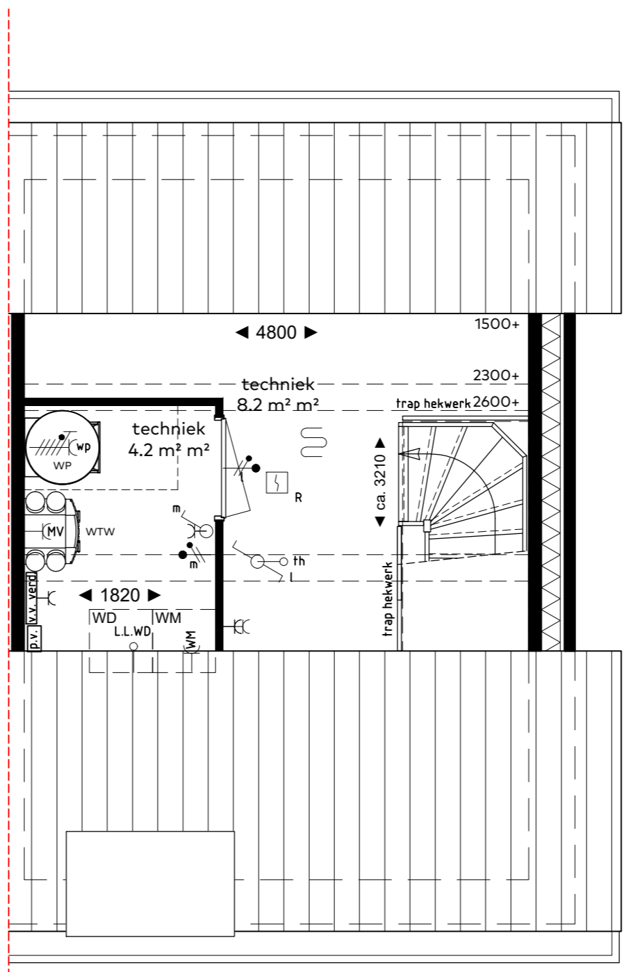
ZOLDER
